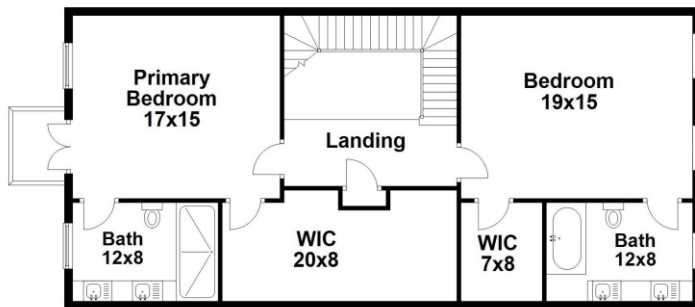
second level
