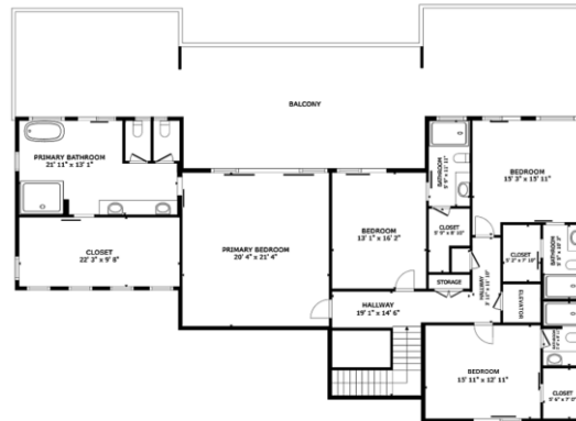
second level
