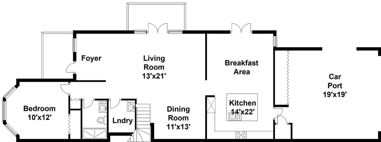
first floor
